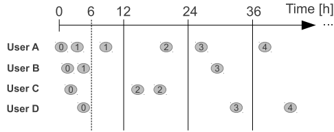
Figure 4: Depiction of our assignment of slices to tweets in the data. Each row corresponds to a user and each oval to a tweet, numbered with the time slice it belongs to. All the tweets containing the original URL are assigned to slice t_0 , and must be posted within 6 hours to grant crowd membership to its user. Subsequent tweets are assigned to other slices as per the diagram.
