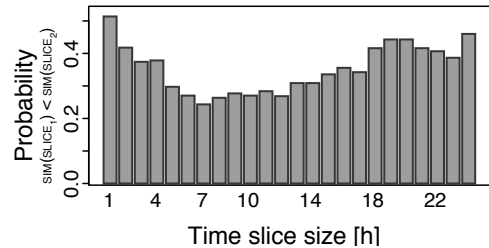
Figure 5: Probability that a crowd’s tweets become more similar on the second time slice (compared to the first time slice) for different choices of time granularity.
